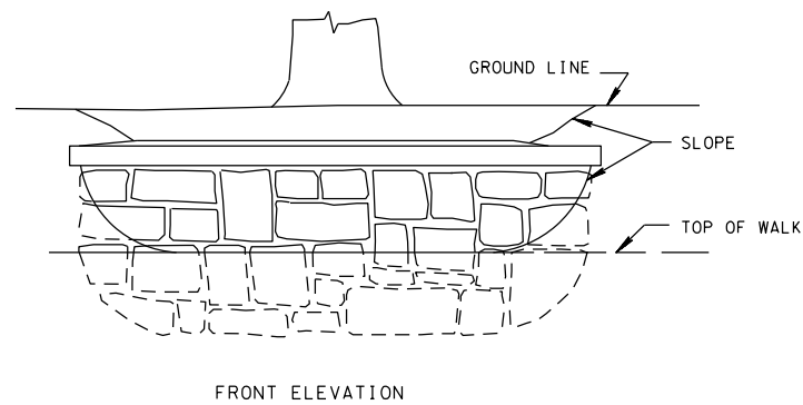
STONE MASONRY TREE WALL
